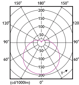
Light Distribution Diagram - EcoHome LEDBulb 16W E27 6500KHV 1PF/20AR
