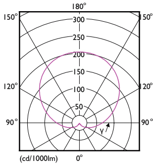
Light Distribution Diagram - EcoHome LEDBulb 7W E27 6500KHV 1PF/20AR
